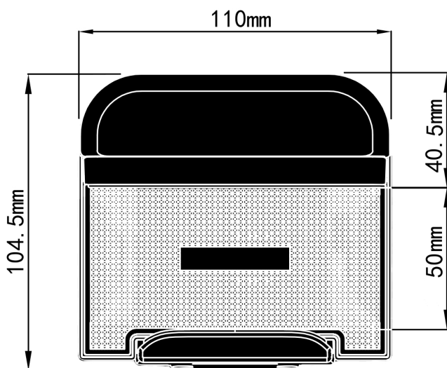
Fig. 3-2 Front View of Display 90E Dimensions
